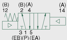
double air pilot 2 position 4-way spring offset no override
